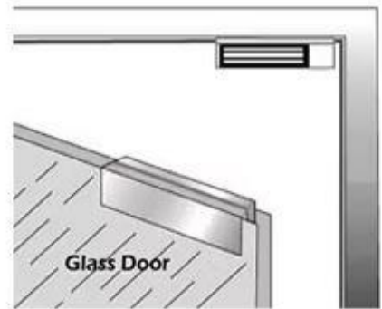
U Type Bracket for Frameless Glass door
